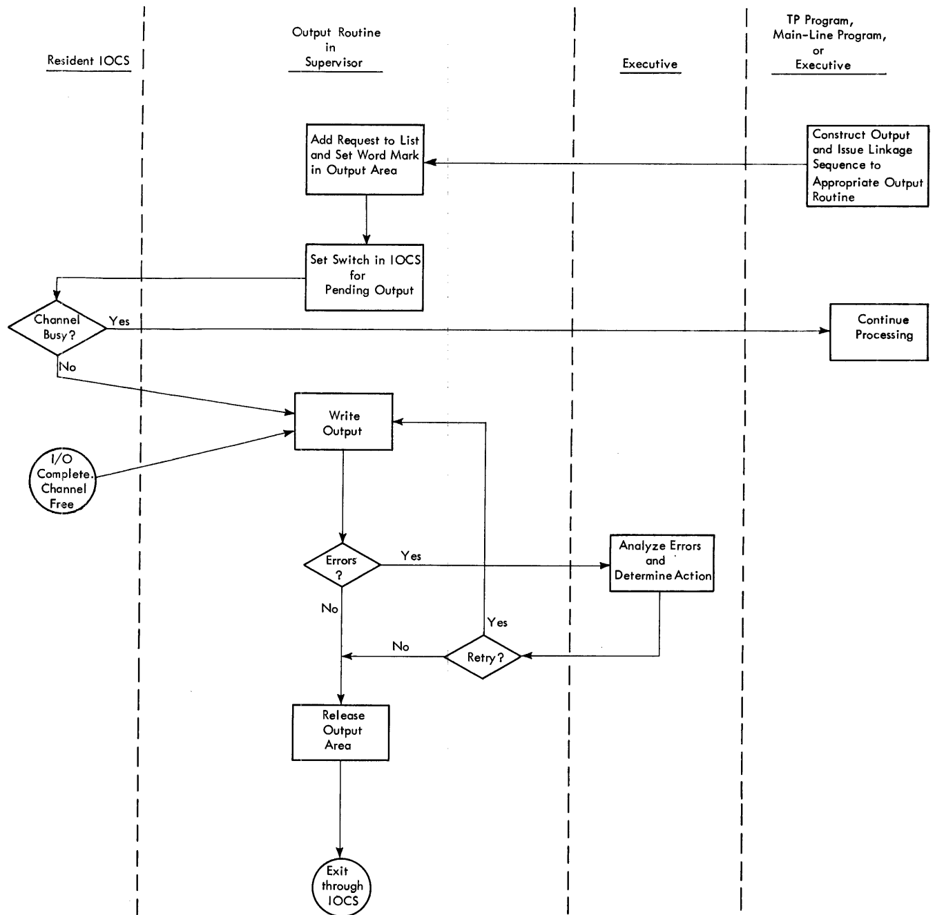
Figure 3. Output Logic
