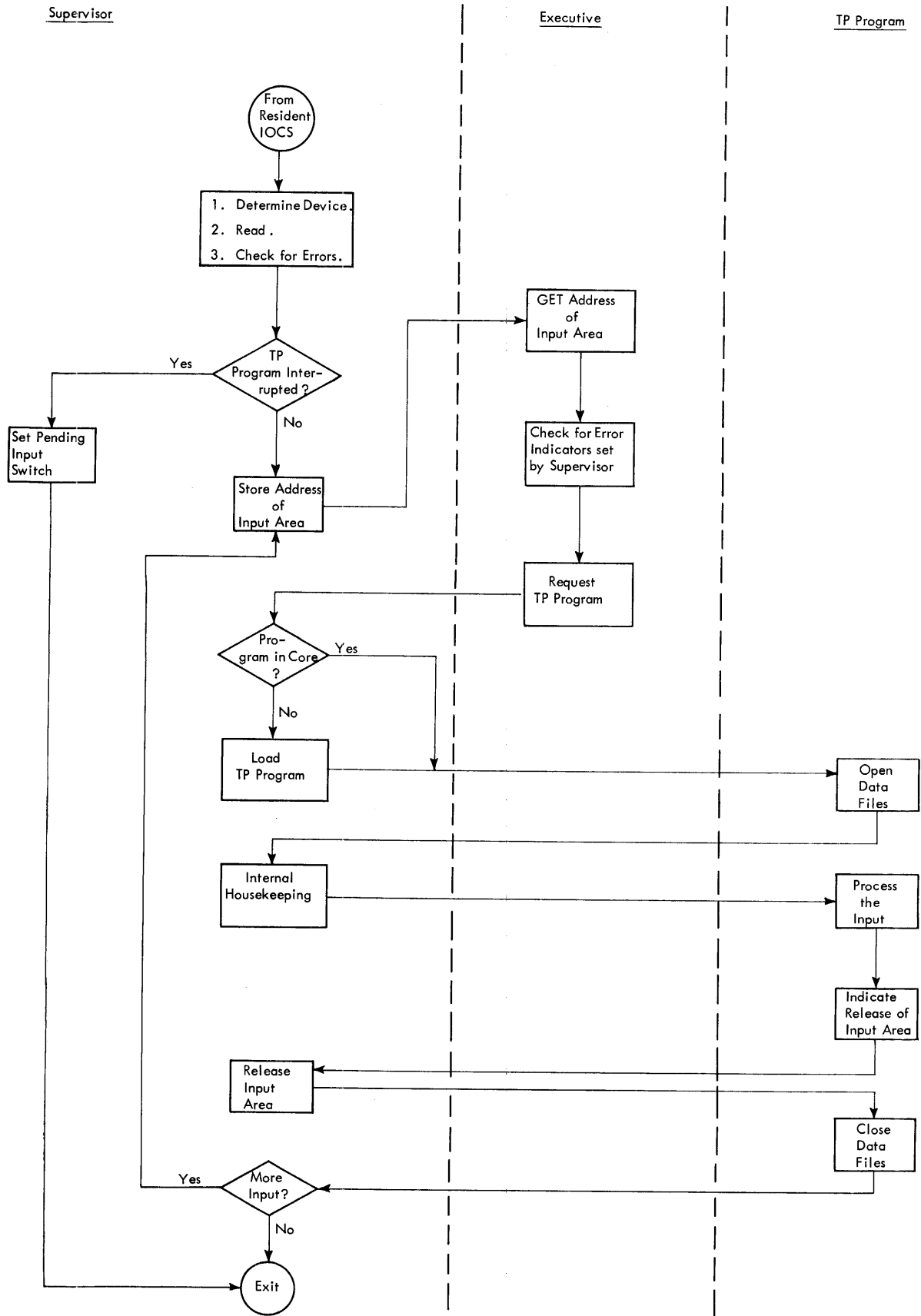
Figure 2. Input Logic
